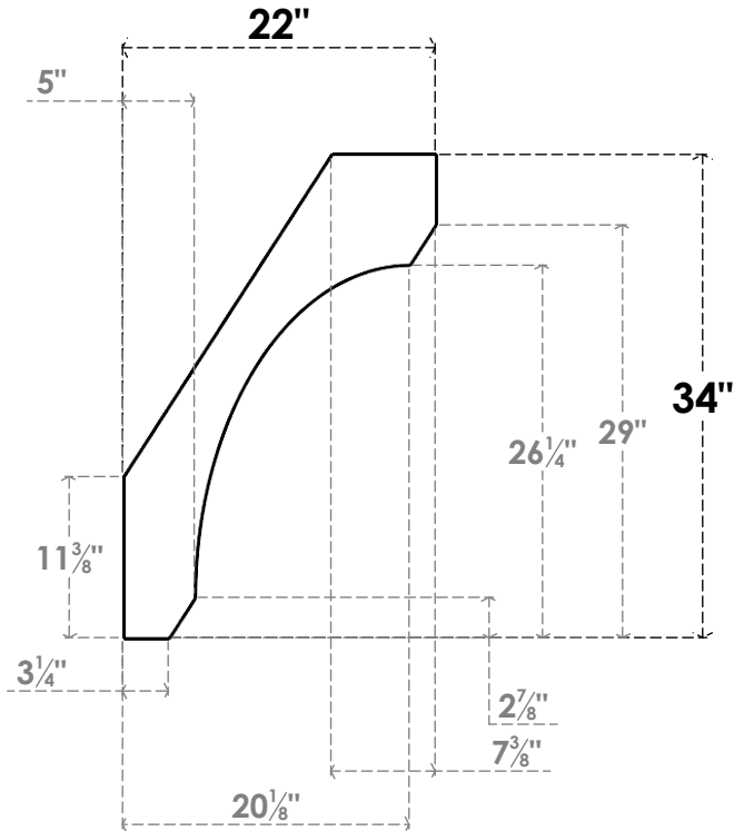
SIDE PROFILE
